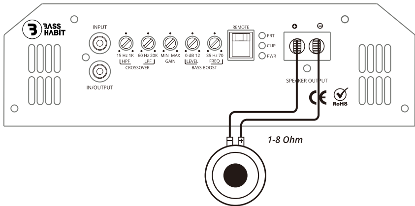
FIG 2: SPEAKER CONNECTIONS
